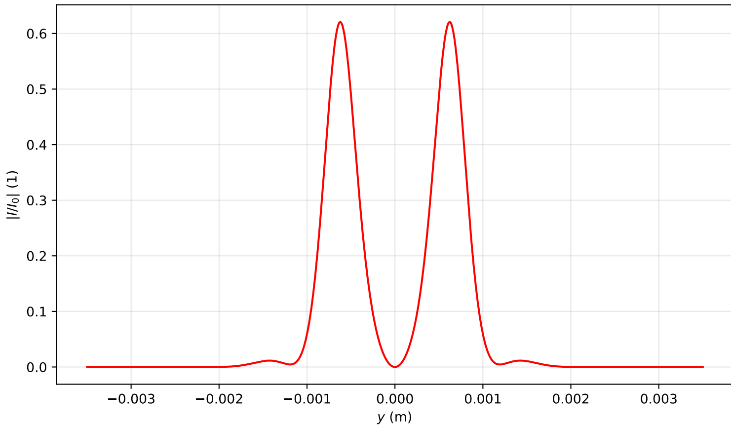
Intensity profile I(x=0, y, z=1.194)/I_0 , P_{in}=5.0P_{cr} , artificial time
